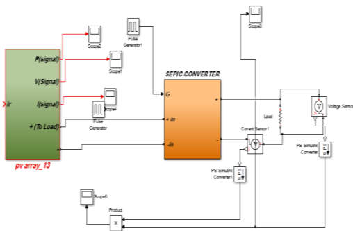
Fig. 3 : MatLab Simulation PV System Model
