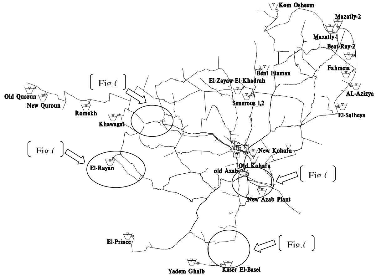
Fig.(1) The Fayoum water distribution network and The location of treatment plants
