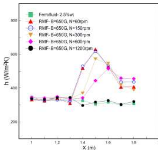
Fig. 10. Effect of rotating magnetic field (uni-pole) on local heat transfer coefficient at different rotating speeds for ferrofluid with 2.5% (wt) at B = 650 G and Re = 2000 .
