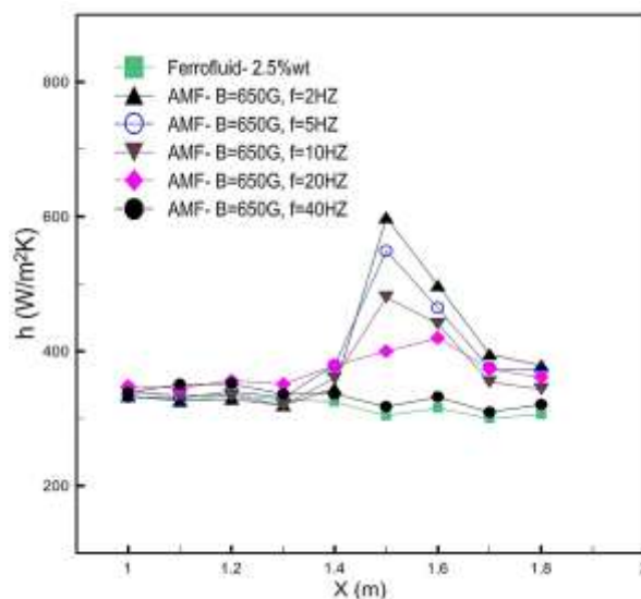
Fig. 9. Effect of alternating magnetic field (uni-pole) on local heat transfer coefficient at different frequencies for ferrofluid with 2.5% (wt) at B = 650 G and Re = 2000 .
