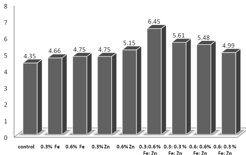
Figure 1. Influence of spraying zinc, Fe on concentrations of carotenoids of safflower petals.
