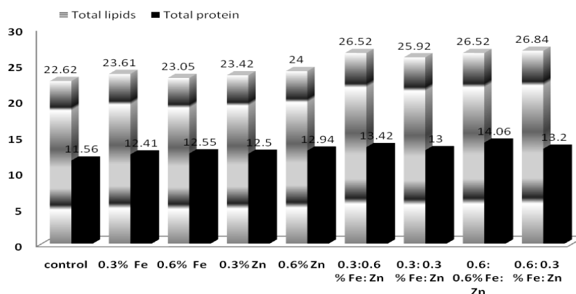
Figure 2 : Influence of spraying Zn, Fe on concentrations of Total lipids and protein (%) of Carthamus tinctorius L seeds.
