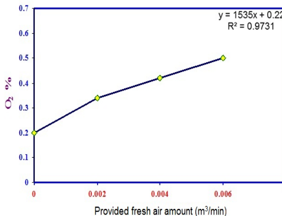
Fig. (14): O 2 percentage as affected sawdust by provided air amount.
