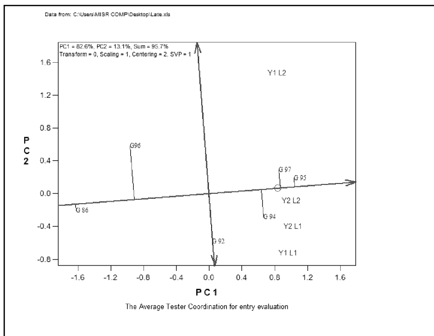
Fig. 1: Average environment coordination (AEC) view of the GGE-biplot for the means performance and stability of varieties.
