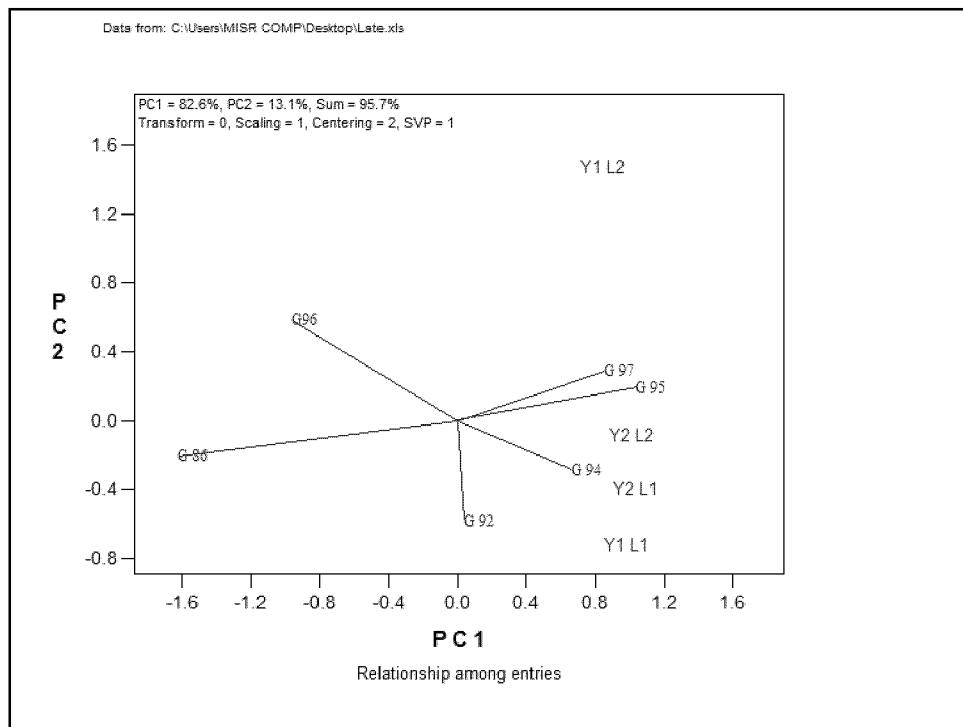
Fig. 3: Biplot of relationships among six varieties in four environments.
