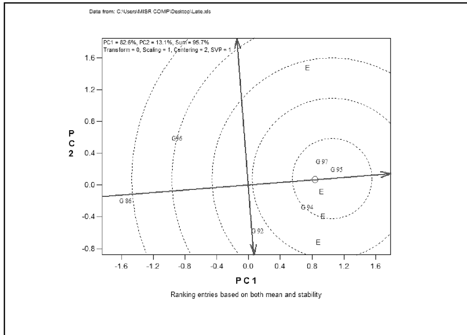
Fig. 2: Ranking of varieties based on both mean and stability refers to ideal varieties.
