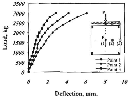
Fig. (7) Experimental Load - Deflection Relationship of Plate HSF3
