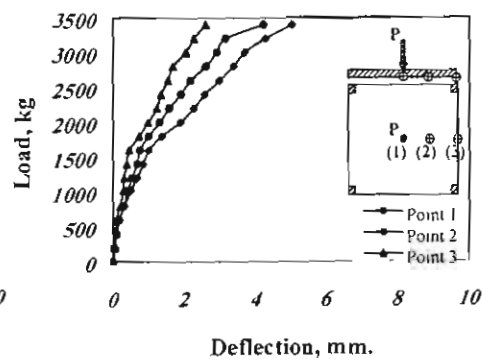
Fig. (12) Experimental Load - Deflection Relationship of Plate HSR5
