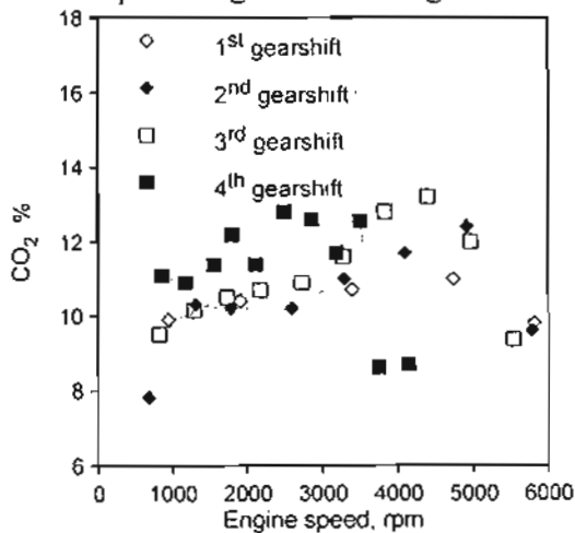
Fig. 8 Emission of carbon dioxide at different engine speed and gearshift.
