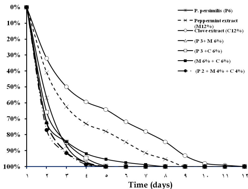
Figure 3: Shows the reduction percentages of spider mite species, T. urticae under different treatments
