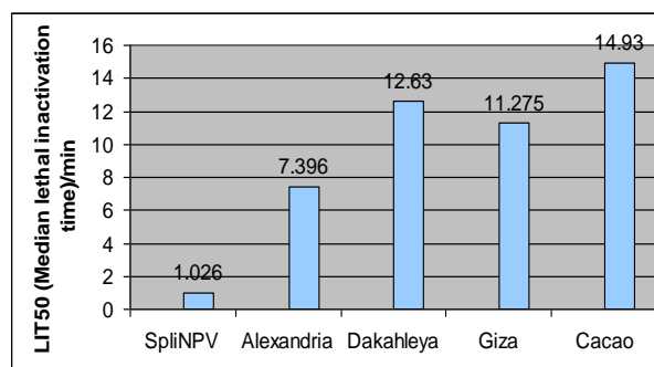
Figure (4) LIT 50 (Median lethal inactivation time) among S littoralis neonate larvae treated with Spli NPV either alone or in combination with propolis isolates or cacao at 1% concentration, all exposed to different UV irradiation periods.
